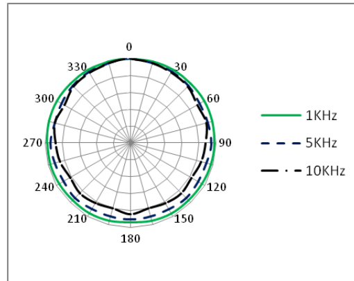
Polar pattern
